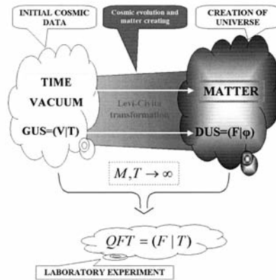
Figure 3: This figure, taken from, 36 shows the quantum creation of the universe in the field reality out of the time \eta=T (right) and in the geometric reality without matter (left). The Hubble law \varphi(\eta) , and creation of matter from vacuum with particle density n(\eta) ( n(0)=0 ) are described as pure relativistic effects by the geometrization of the energy constraint. Only in the limit of tremendous energy of the Quintessence there does appear a possibility of describing the universe as the Newton-like system F(\eta) .
