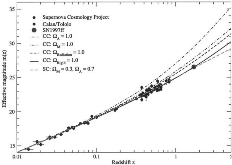
Figure 1: The Hubble diagram in cases of the absolute units of standard cosmology (SC) (4) and the relative ones of conformal cosmology (CC) (2). 18 The points include 42 high-redshift Type Ia supernovae and the reported farthest supernova SN1997ff. 19 The best fit to these data requires a cosmological constant \Omega_\Lambda = 0.7 \Omega_{\text{ColdDarkMatter}} = 0.3 in the case of SC, whereas in CC these data are consistent with the dominance of the rigid state (6).
