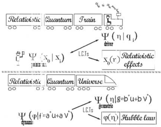
Figure 2: At the top of figure, a relativistic train is depicted with an unstable particle. The lifetime of this particle is measured by two Einstein observers, by a pointsman and a driver, who communicate to each other their measurement outcomes on the phone. Each of the observers has his world space of events, his time (pointsman - variable X_0 , and driver - geometrical interval t ) and his notebook, as a wave function of a particle in terms of amplitudes of probability to find a particle at an arbitrary point of the world space, if at the initial moment its initial data are given. At the bottom of the figure there is an image of the universe where each observer has two sets of measurable quantities corresponding to two observers of the particle. To the pointsman there corresponds a field set of measurable quantities (mass j and density of a number of particles n=a_q^+ a_q with a set of quantum numbers q ), and to the driver, the geometrical set of measurable quantities (time interval h and initial data of the density of the Bogoliubov b_q, b_q^+ quasiparticles ). 31
